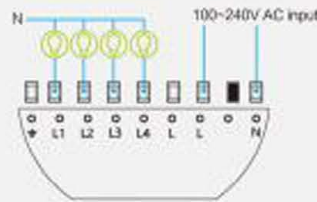
High Power Lighting Wiring Diagram 1-1
