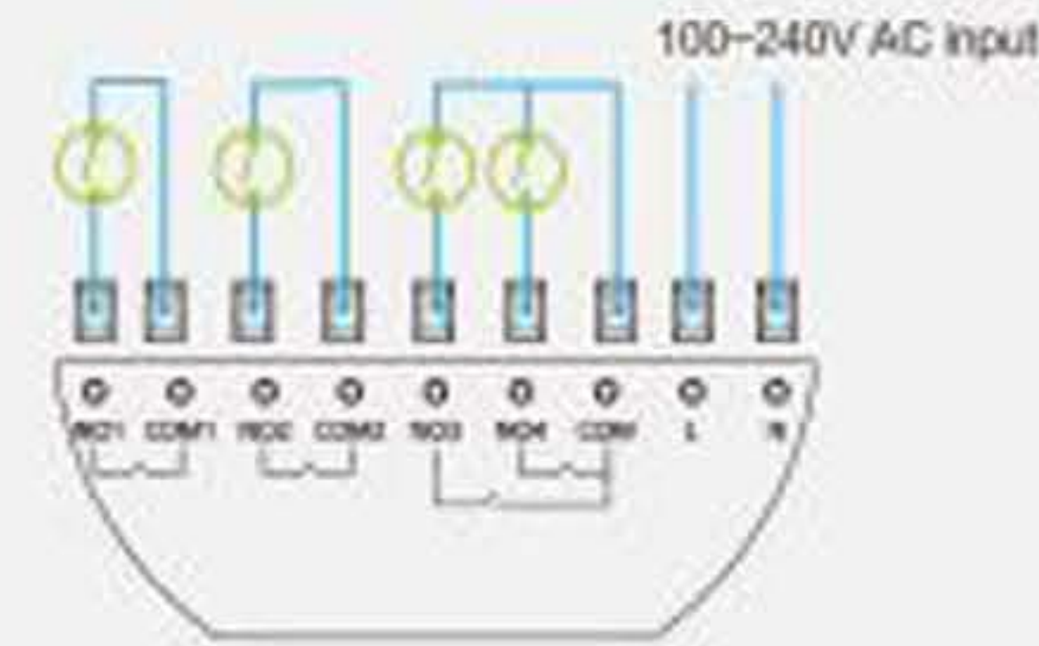
Dry Contact Or Weak Voltage Control Lighting Wiring Diagram 1-2
