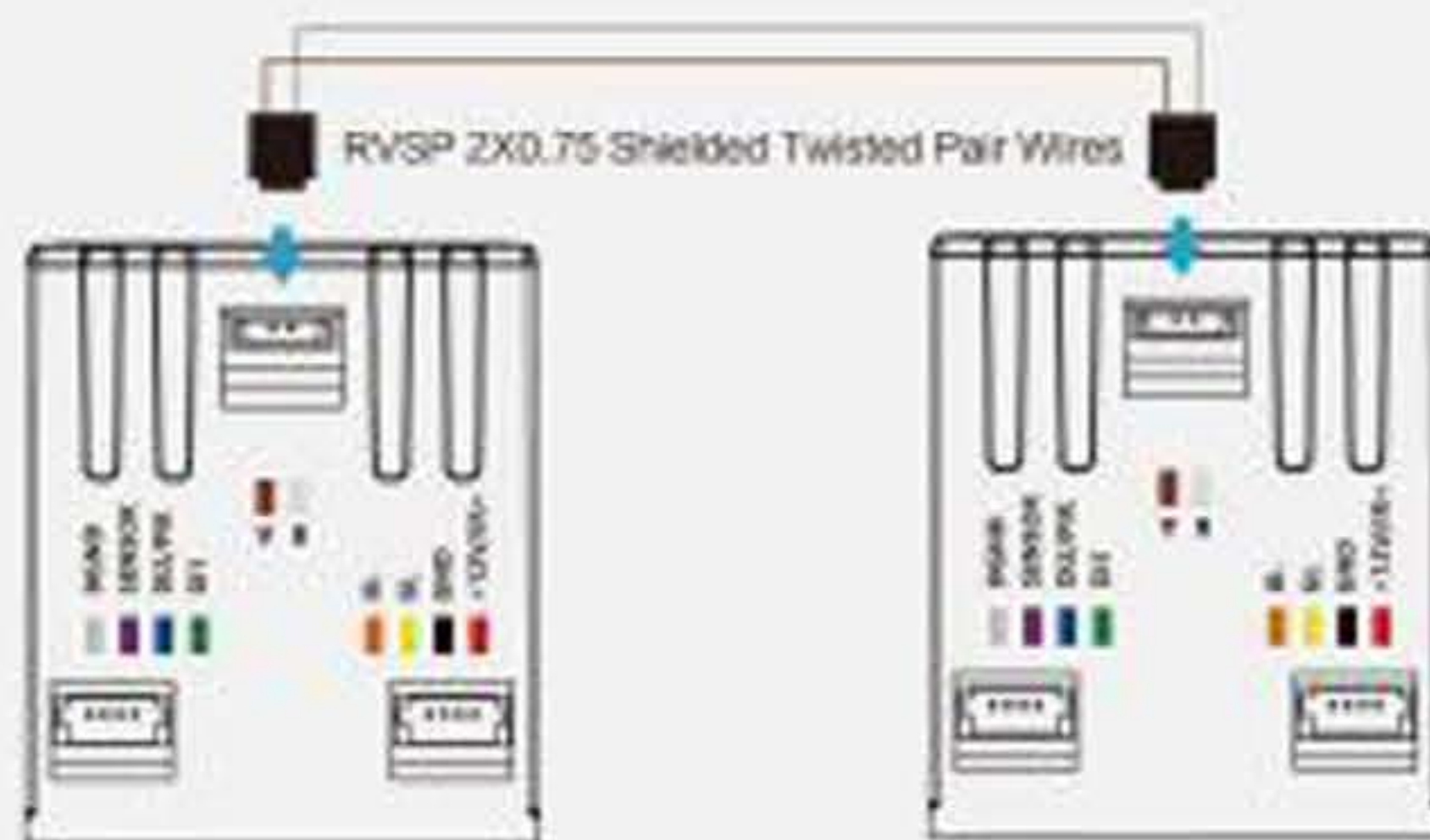
Wired RS485 Wiring Diagram 2-1
