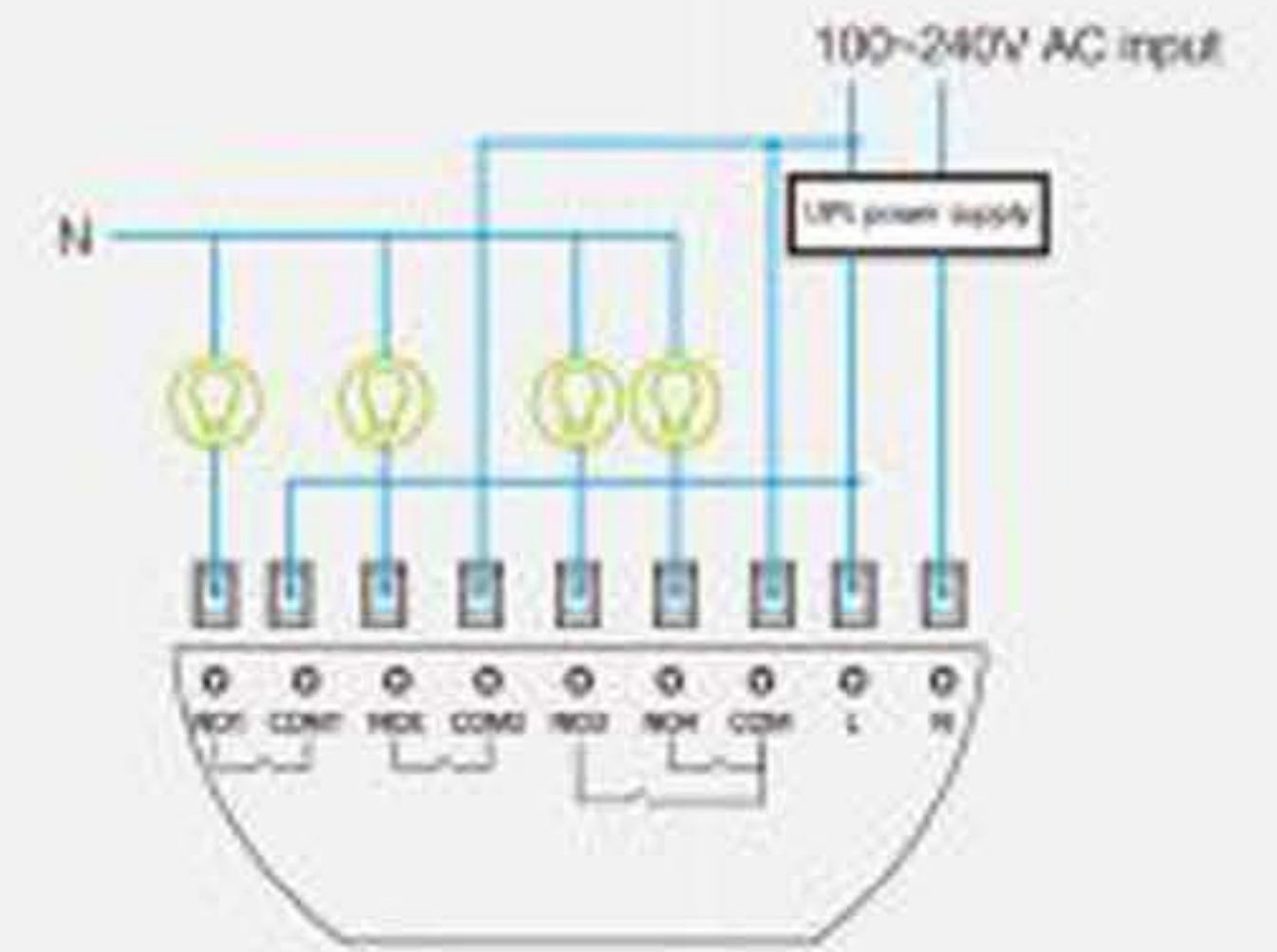
Emergency Control Lighting Wiring Diagram 1-3
